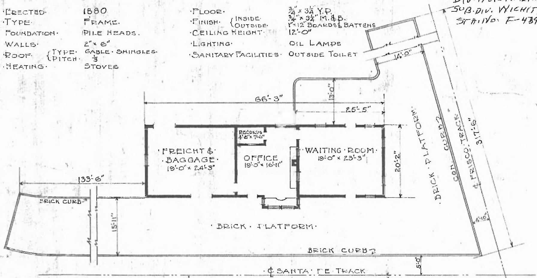
·FLOOR PLAN· SCALE \frac{1}{16} " = 1'-0"
