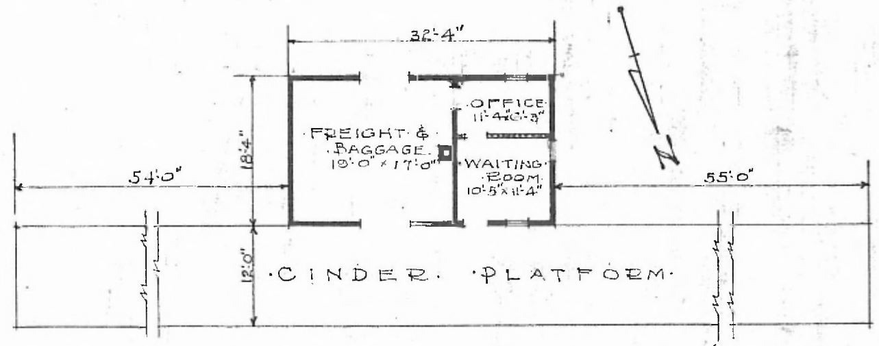
·FLOOR PLAN· SCALE 1/16" = 1'0"
