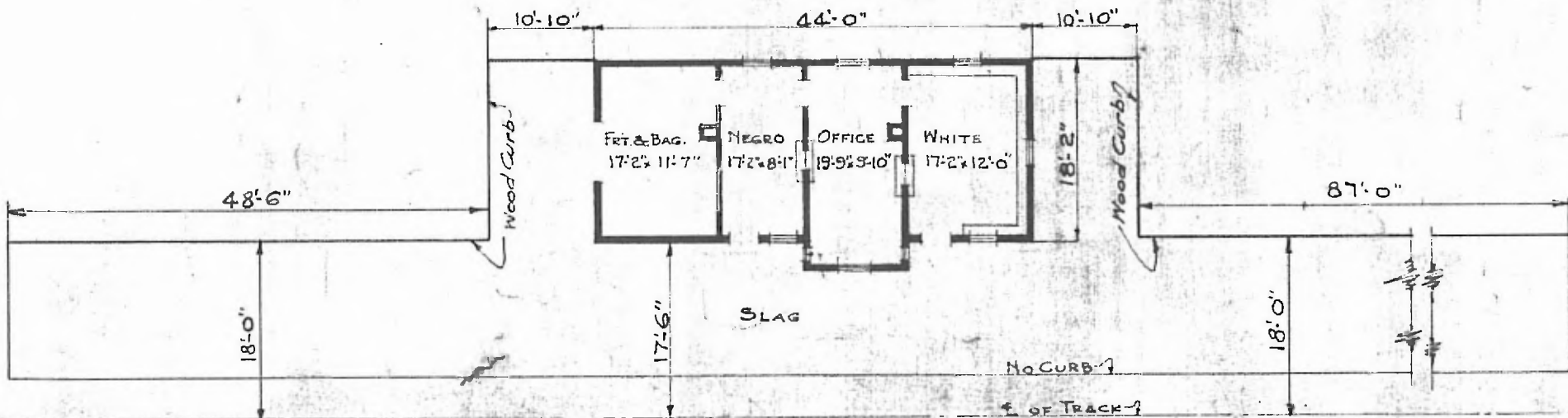
FLOOR PLAN SCALE: \frac{1}{16} = 1'-0"
