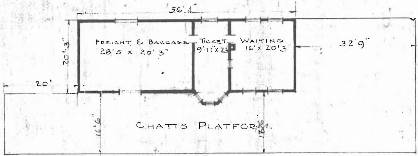
FLOOR PLAN SCALE 1/16" = 1'-0"
