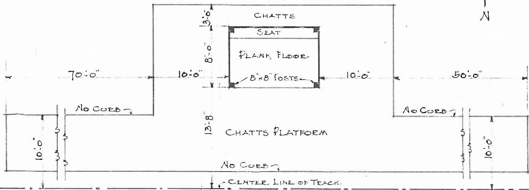
FLOOR PLAN. SCALE \frac{1}{8}'' = 1'-0'' .
