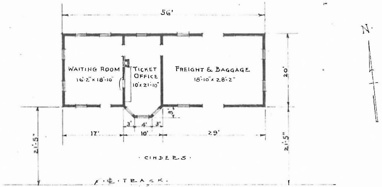
FLOOR PLAN SCALE: 1/16" = 1'-0"
