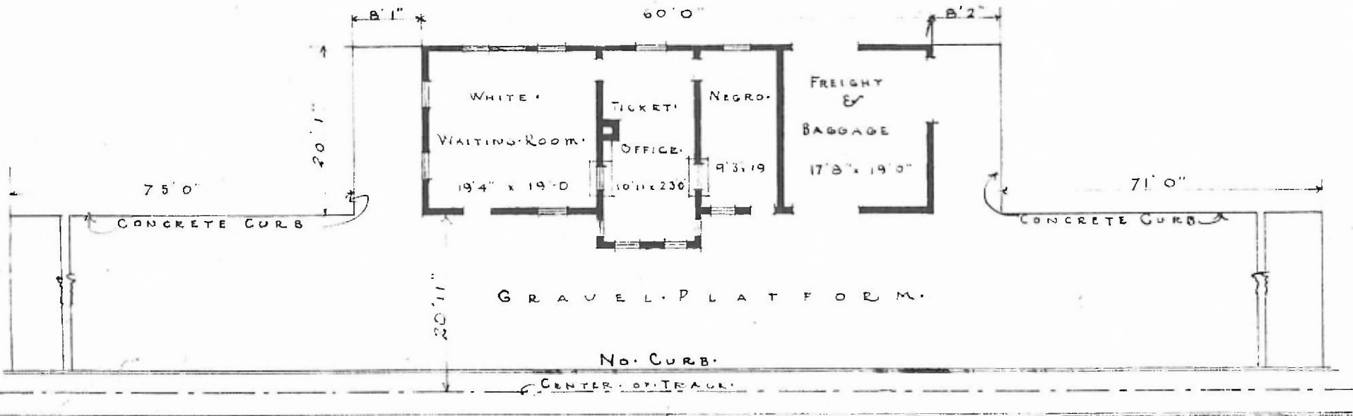
FLOOR PLAN SCALE \frac{1}{16} = 1'
