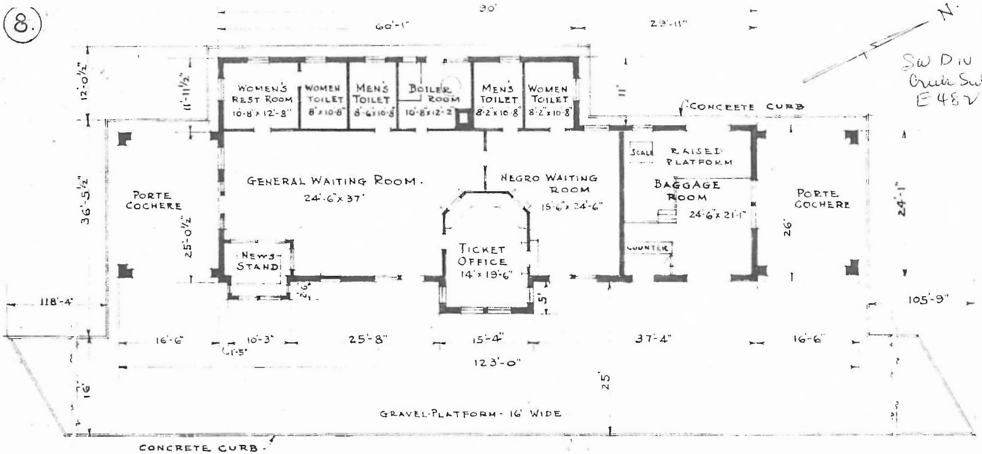
FLOOR PLAN. SCALE: 1/16" = 1'-0"
