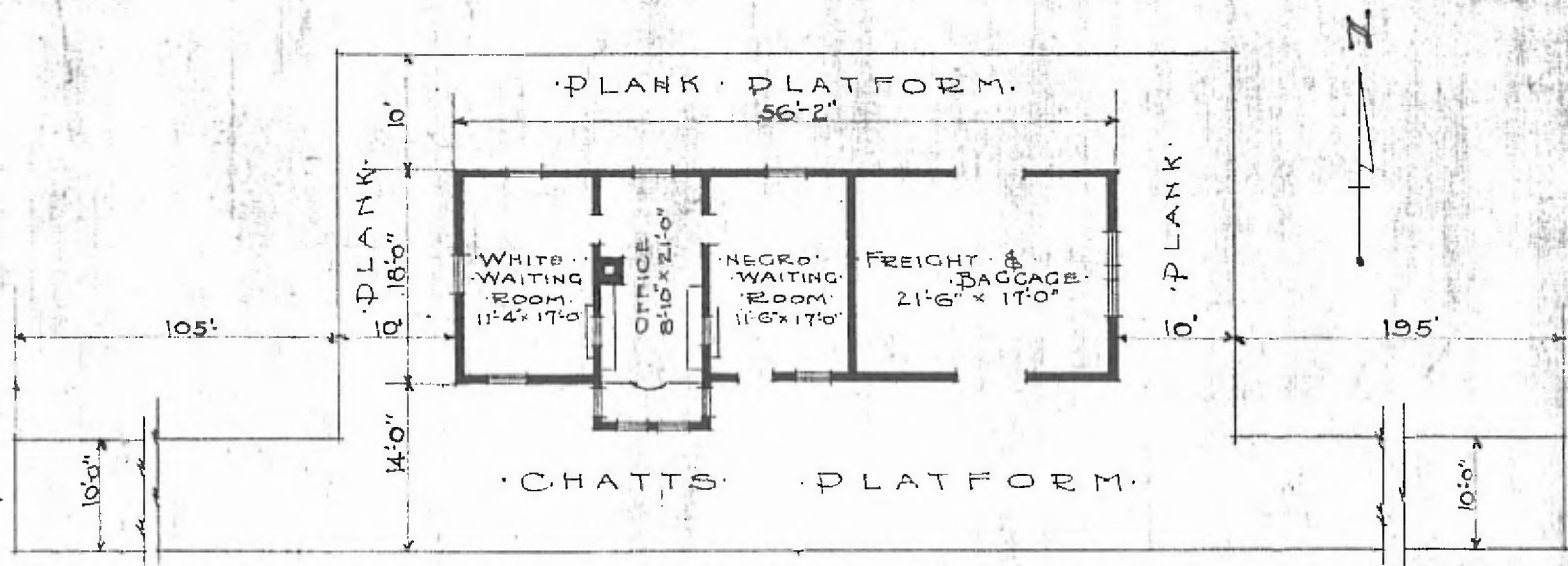
·FLOOR PLAN· ·SCALE \frac{1}{16} " = 1'-0".
