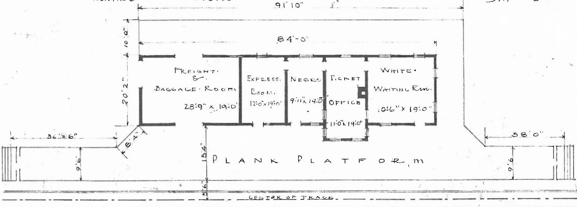
- FLOOR PLAN - Scale \frac{1}{16} = 1'0"
