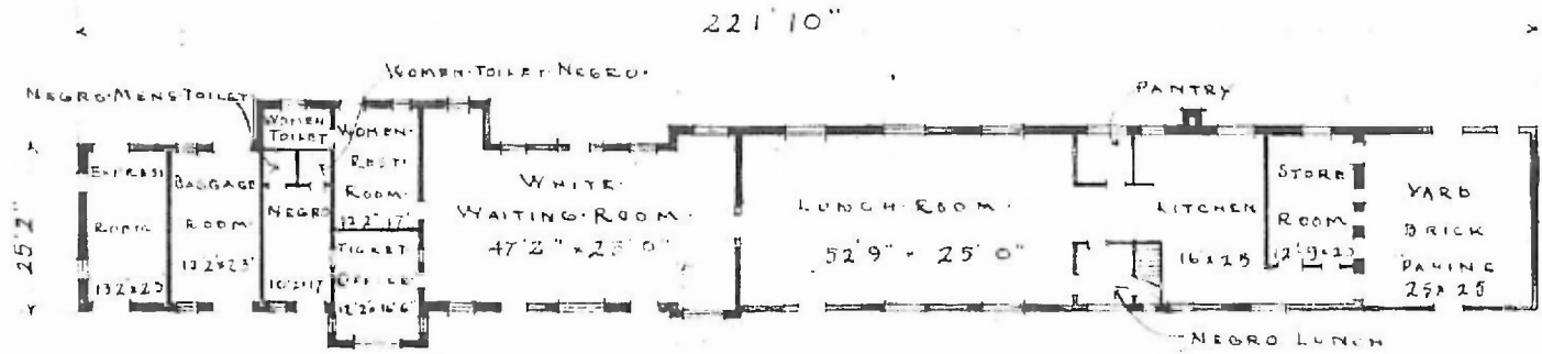
- FLOOR PLAN - SCALE \frac{1}{32} = 1'0"
