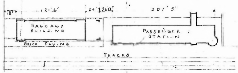
PLOT PLAN SCALE 1" = 100'
