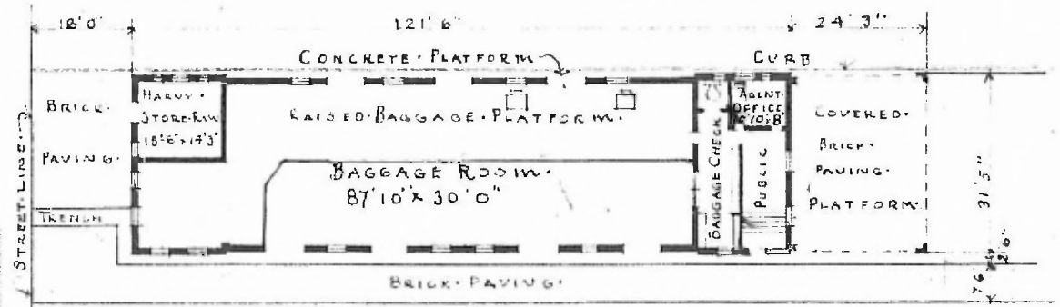
FLOOR PLAN SCALE 3/32" = 10'
