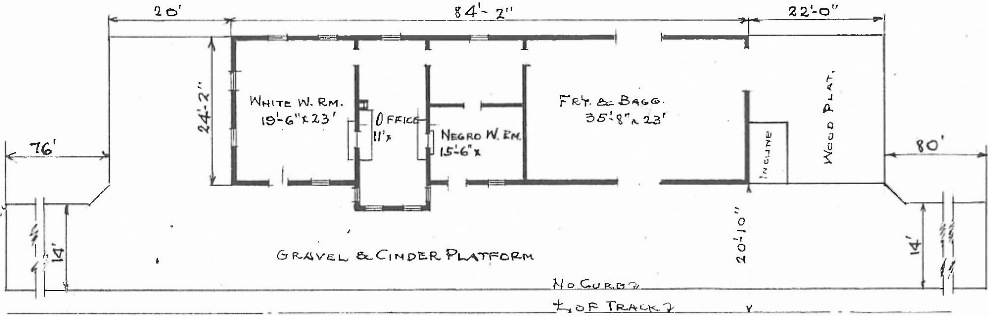
FLOOR PLAN SCALE: \frac{1}{16} " = 1'-0"
